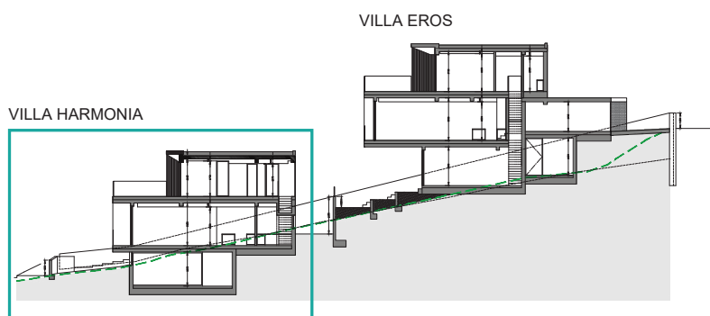
2 SECTION B-B 1:200
